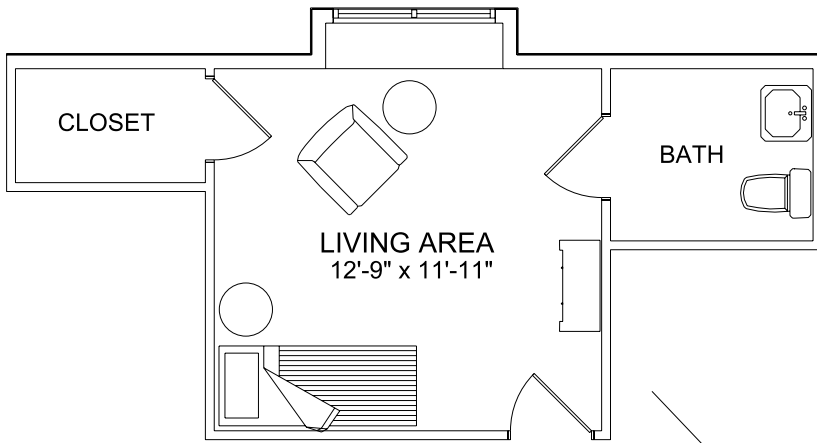
INDIVIDUAL STUDIO ENLARGED VIEW
